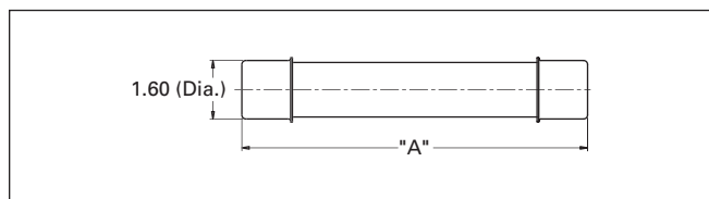
Figure 5-2. NCLPT Fuse Dimensional Details — Inches
