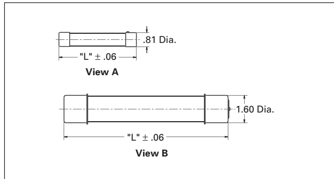
Figure 5-1. CLPT Fuse Dimensional Details — Inches
