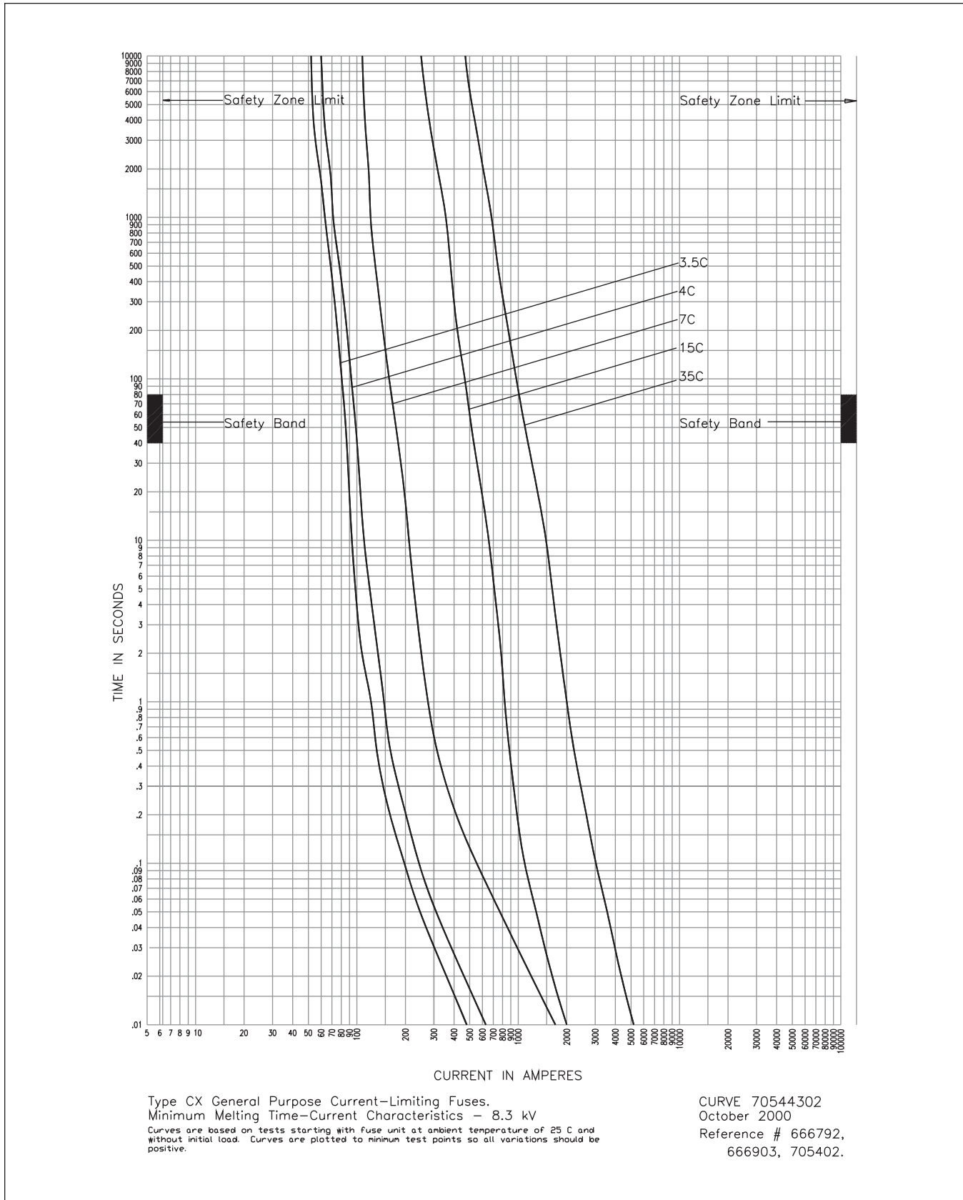
Figure 7-20. Curve Number 70544302
