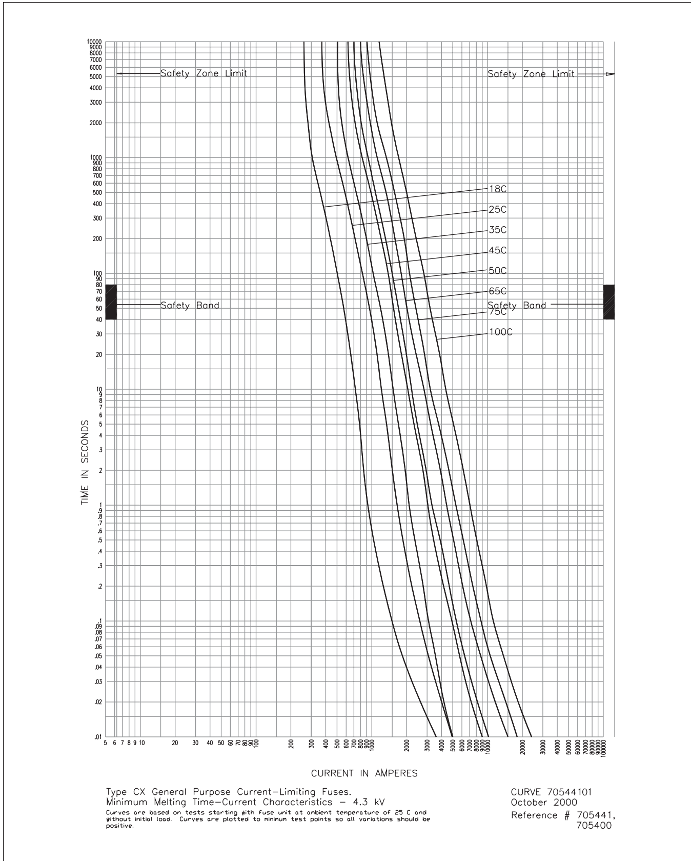
Figure 7-8. Curve Number 70544101
