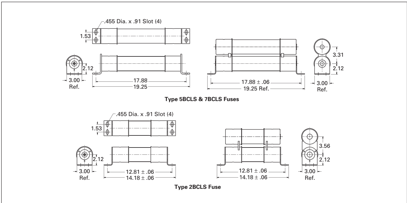
Figure 4-5. BCLS Fuse Dimensional Details
