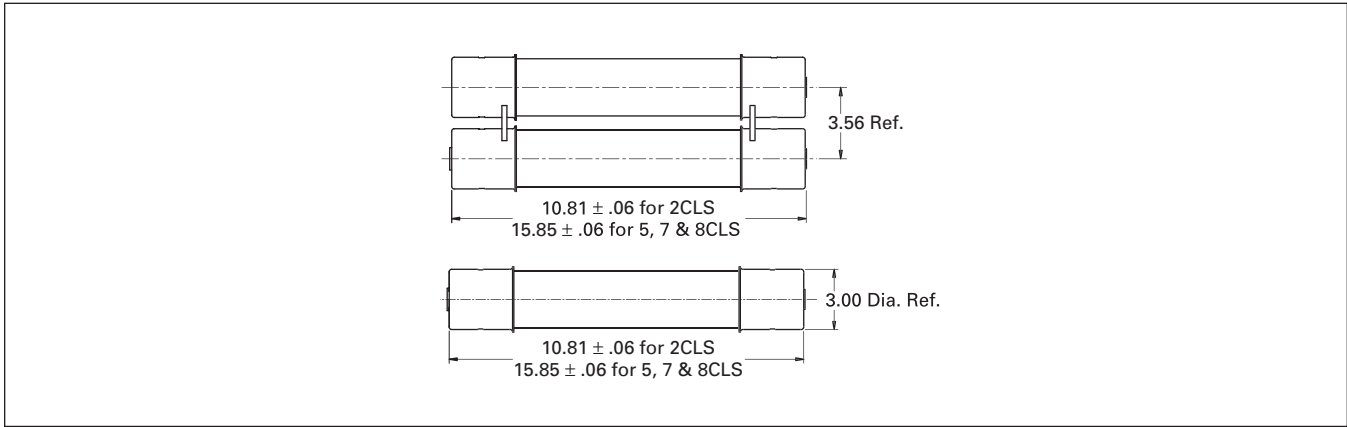
Figure 4-4. CLS Fuse Dimensional Details
