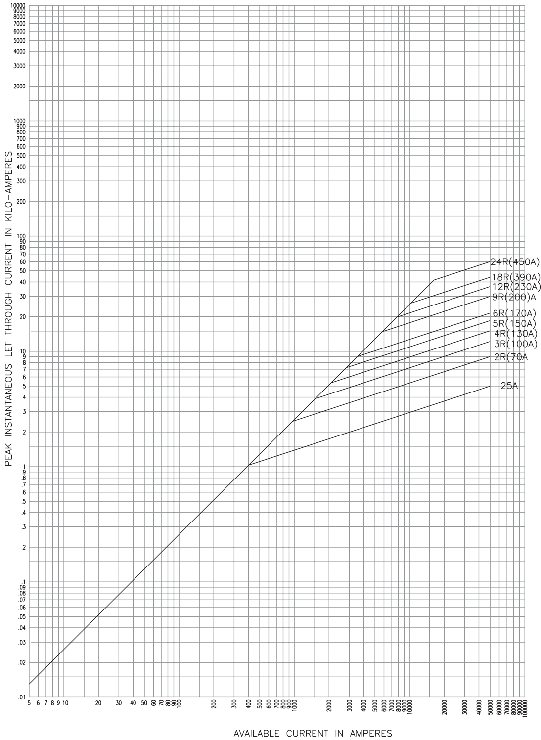
Type CLS2-25A, 2R thru' 24R Motor Start Current Limiting Fuses. Peak let Through Current Characteristics - 2.4 kV Curves are plotted to maximum test points so all variations should be negative.
