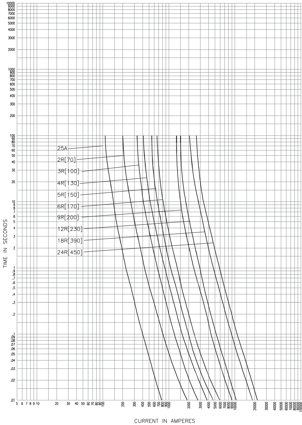
Type CLS2 - 25A, 2R thru' 24R Motor Start Current Limiting Fuses. Total Clearing Time-Current Characteristics - 2.4 kV Curves are based on tests starting with fuse unit at ambient temperature of 25 C and without initial load. Curves are plotted to maximum test points so all variations should be negative.
