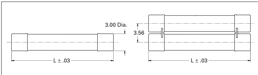
Figure 3-5. HLE Fuse Dimensional Details — Inches
