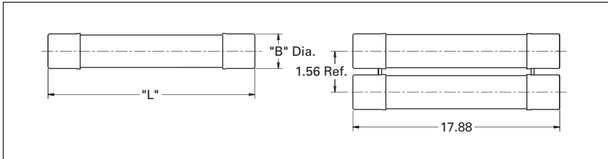
Figure 3-4. CLE Fuse Dimensional Details — Inches
