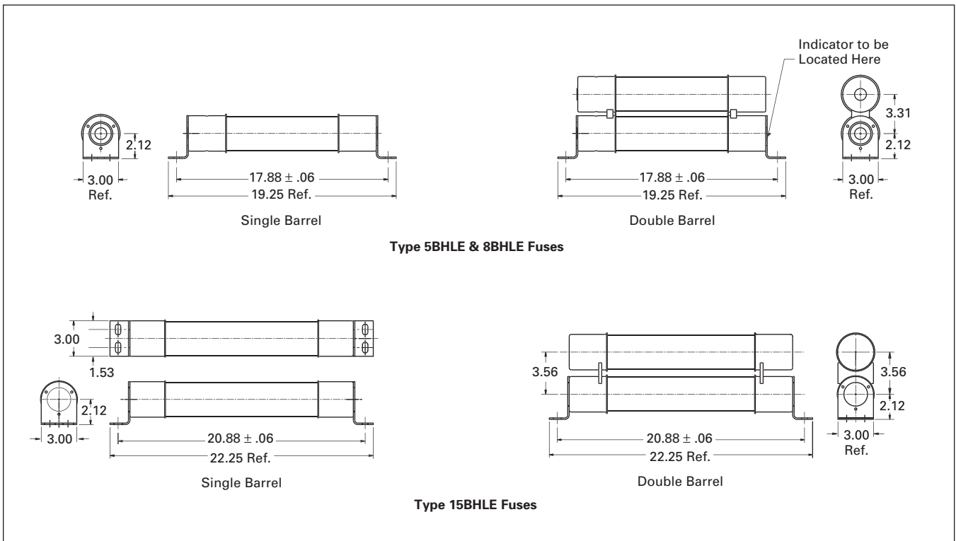
Figure 3-6. BHLE Fuse Dimensional Details — Inches
